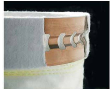
The unique shape of the ProSnap's band is key to its superior qualities.
