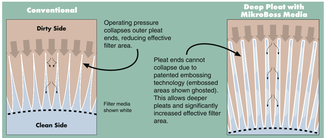
This illustration represents the media at full size, with conventional 1.25" pleats, and Deep Pleat 1.94" pleats, increasing filter area by 55%.
